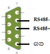
RS485
